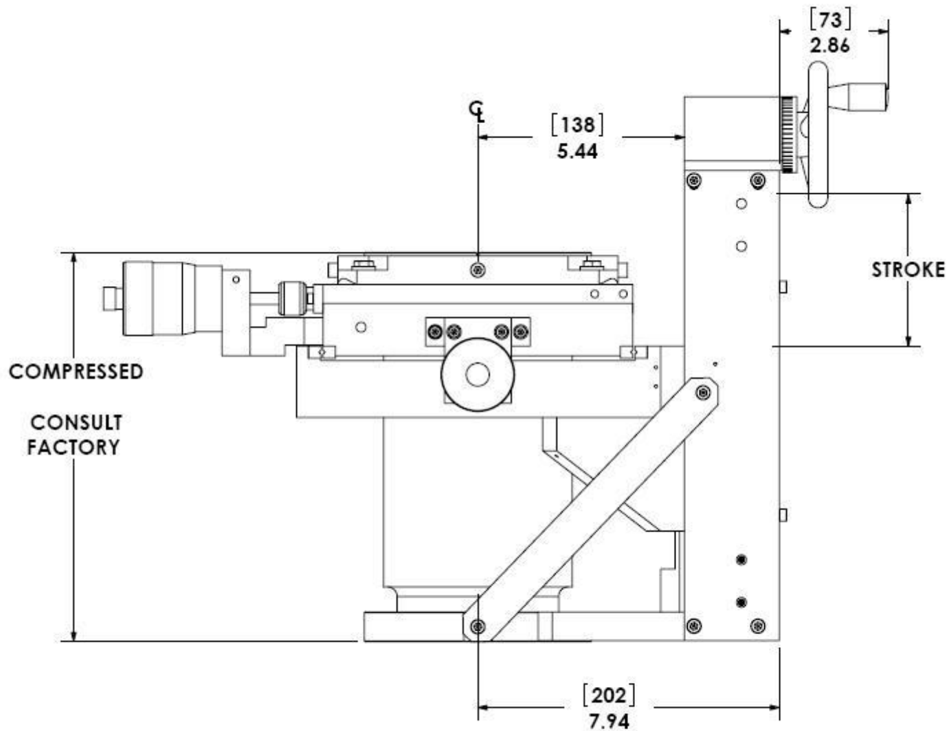
MB2000-1/2 W/LARGE MICROMETERS
